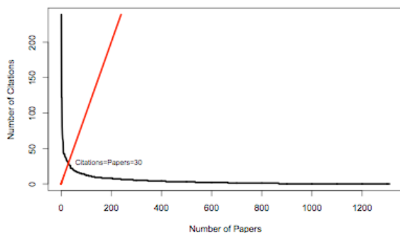
Figure 6. H-index.
