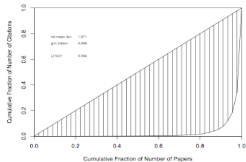
Figure 7. Lorenz Curve.
